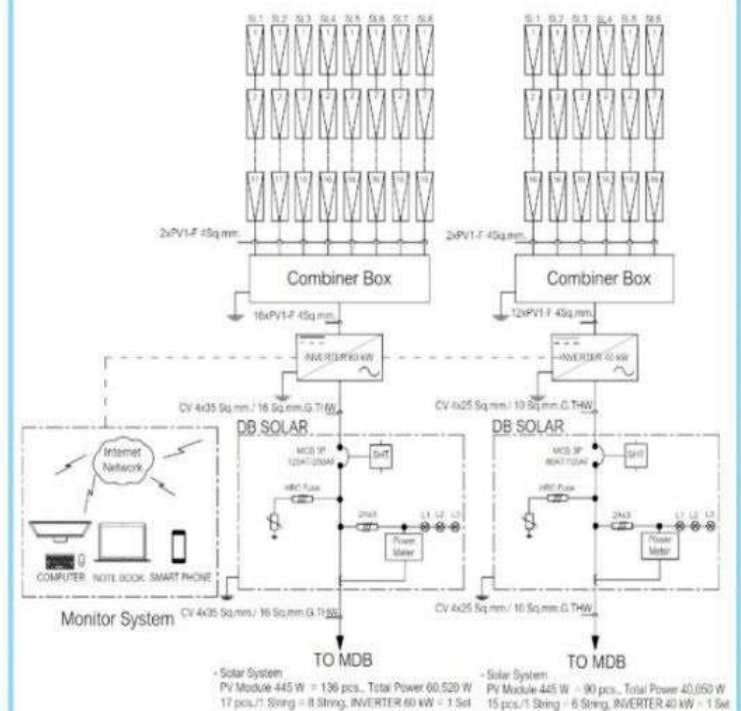
SLD Diagram of 100 KW
